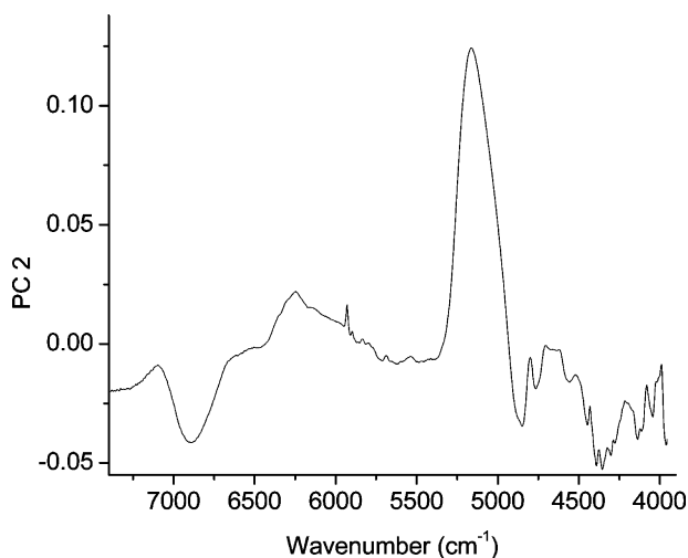
Fig. 5. The 2nd PLS component of untreated NIR data compared with moisture content determined by KF titration is dominated by the water band at around 5160 cm -1 .
