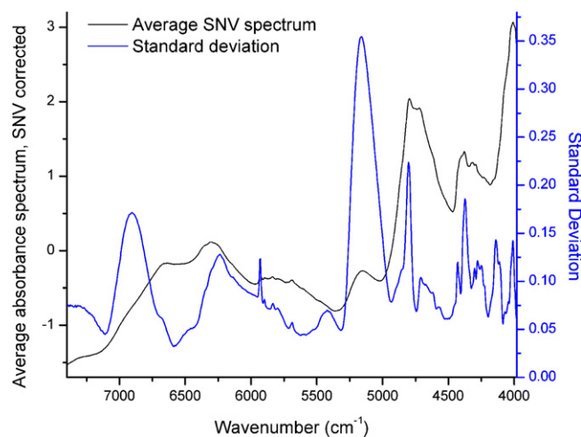
Fig. 2. Standard deviation spectrum for all samples, containing average SNV-corrected spectrum and standard deviation.
