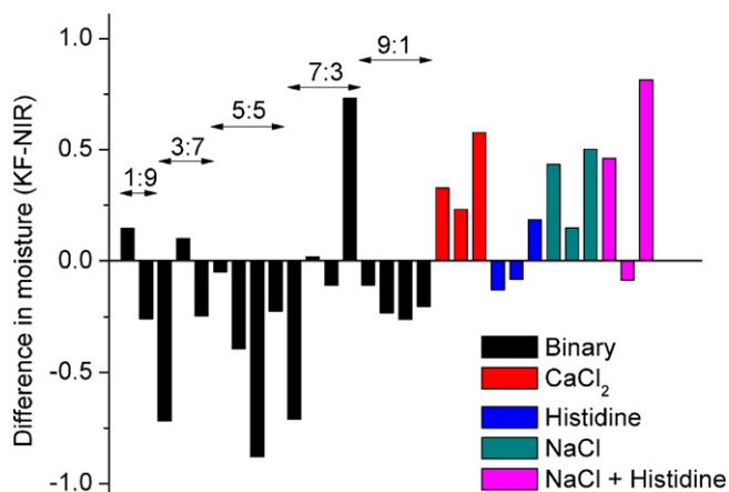
Fig. 8. Differences between estimated moisture content and KF results according to composition. For binary mixtures the mannitol–sucrose ratio is given. All tertiary and quaternary mixtures were based on a mannitol–sucrose ratio of 5:5.
