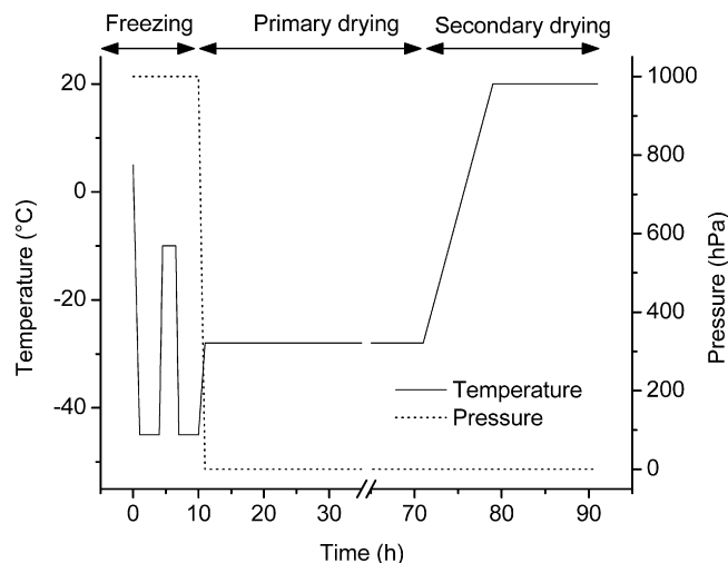
Fig. 1. Overview over the freeze-drying process.
