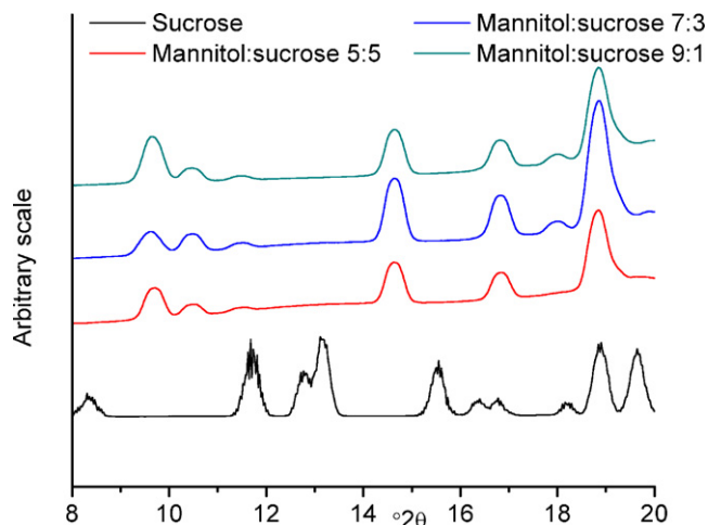
Fig. 4. XRPD diffractogram of sucrose reference and of freeze-dried mannitol–sucrose mixtures with a weight ratio of 5:5, 7:3 and 9:1.
