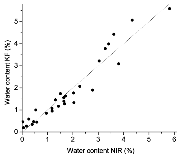
Fig. 6. Comparison of estimated data based on SNV-corrected NIR spectra in the range 4200–7400 cm -1 with obtained KF results.
