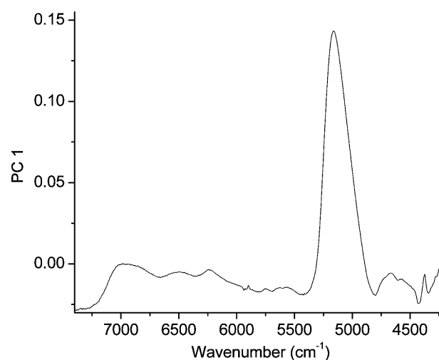
Fig. 7. Loading of PLS component for SNV-corrected NIR data in the range 4200–7400 cm -1 compared to KF data.
